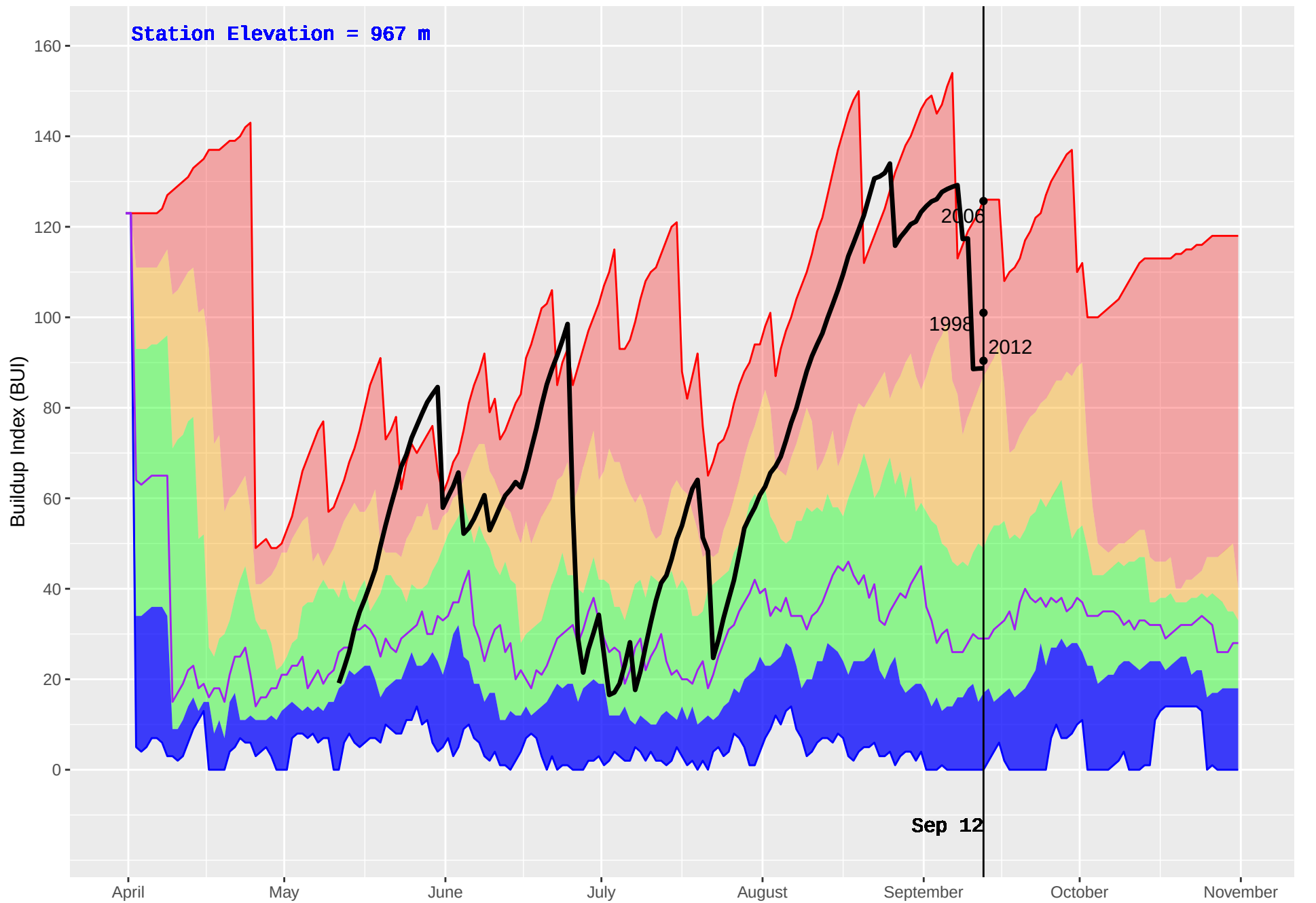
WONOWON (136) : Historical (1990–2016) and Current (2018) Daily Buildup Index (BUI)
